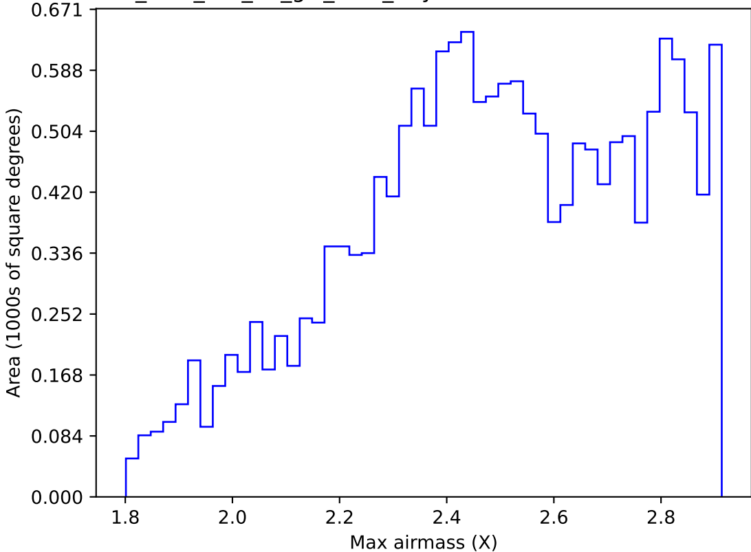
too_elab_r32_d2_giz_v3.4_10yrs WFD z band: Max airmass
