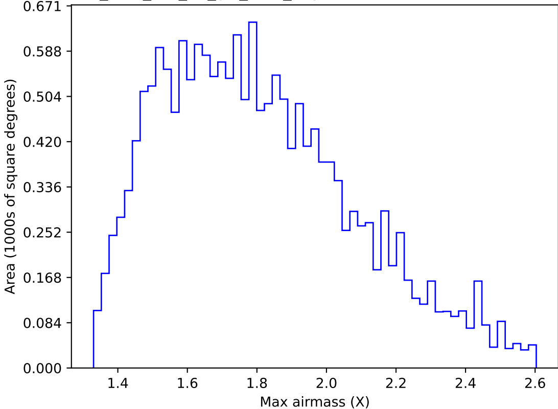
too_elab_r32_d2_giz_v3.4_10yrs WFD u band: Max airmass
