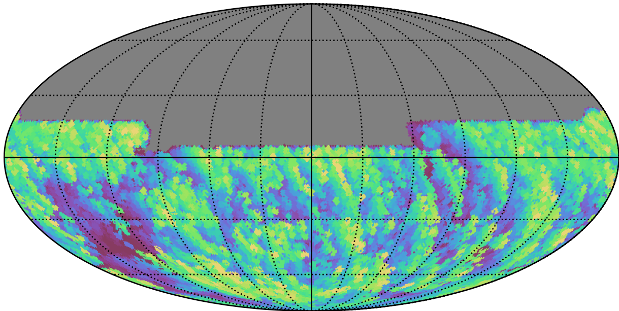
too_elab_r32_d2_giz_v3.4_10yrs All sky y band: Max airmass
