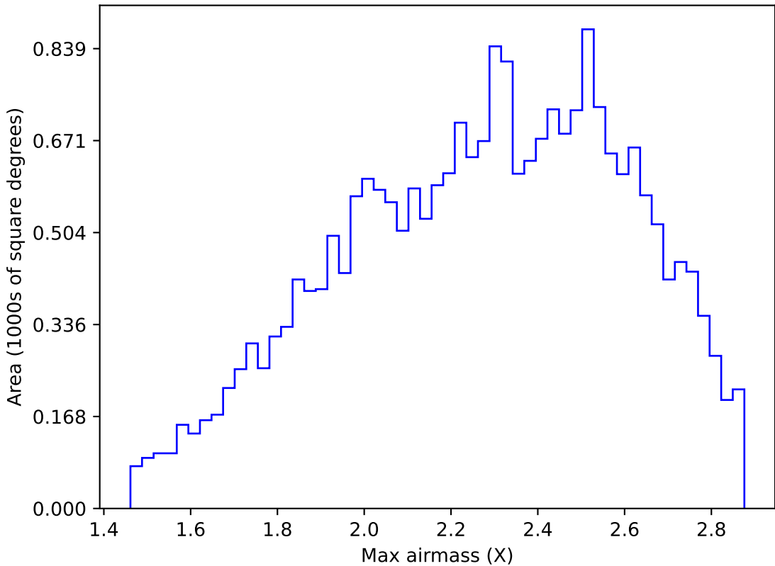
too_elab_r32_d2_giz_v3.4_10yrs All sky y band: Max airmass
