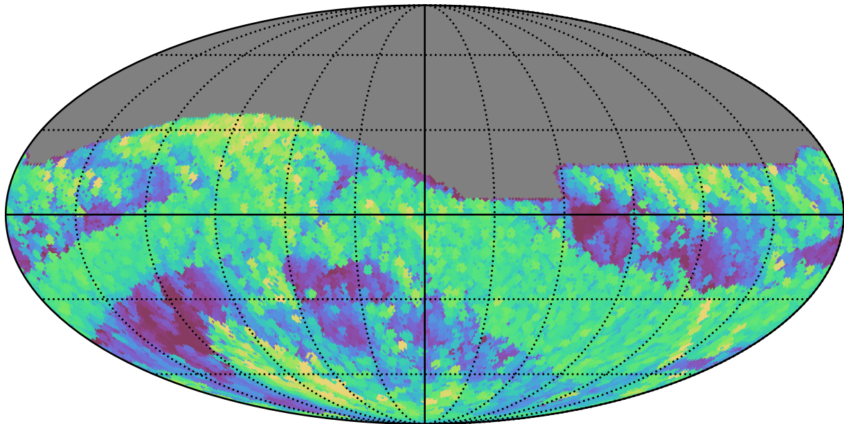
too_elab_r32_d2_giz_v3.4_10yrs All sky r band: Max airmass
