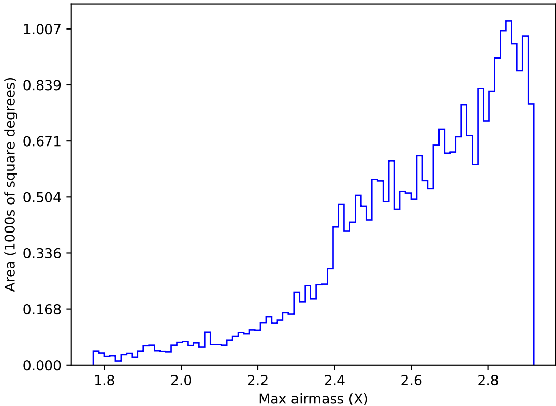
too_elab_r32_d2_giz_v3.4_10yrs All sky all bands: Max airmass
