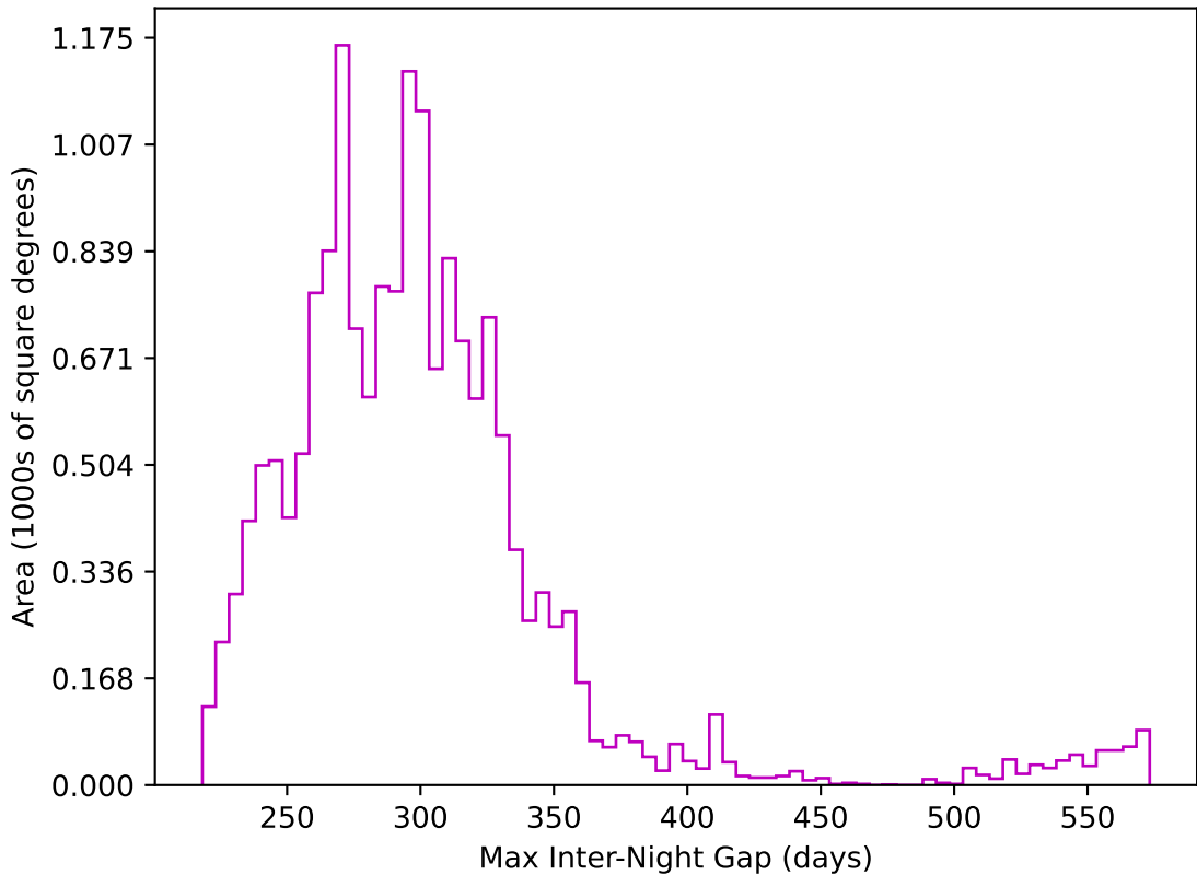
too_elab_r32_d2_giz_v3.4_10yrs WFD z band: Max Inter-Night Gap
