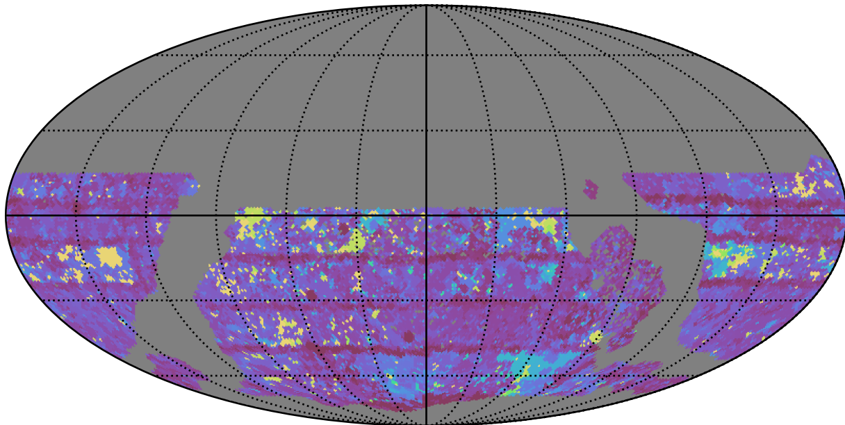
too_elab_r32_d2_giz_v3.4_10yrs WFD y band: Max Inter-Night Gap
