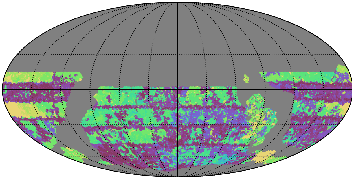
too_elab_r32_d2_giz_v3.4_10yrs WFD u band: Max Inter-Night Gap
