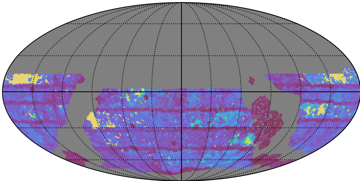
too_elab_r32_d2_giz_v3.4_10yrs WFD r band: Max Inter-Night Gap
