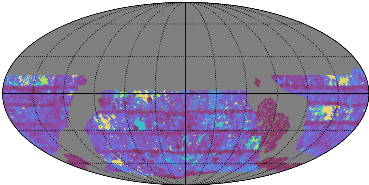
too_elab_r32_d2_giz_v3.4_10yrs WFD i band: Max Inter-Night Gap
