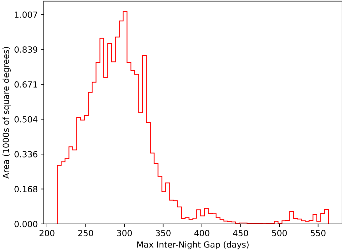
too_elab_r32_d2_giz_v3.4_10yrs WFD i band: Max Inter-Night Gap
