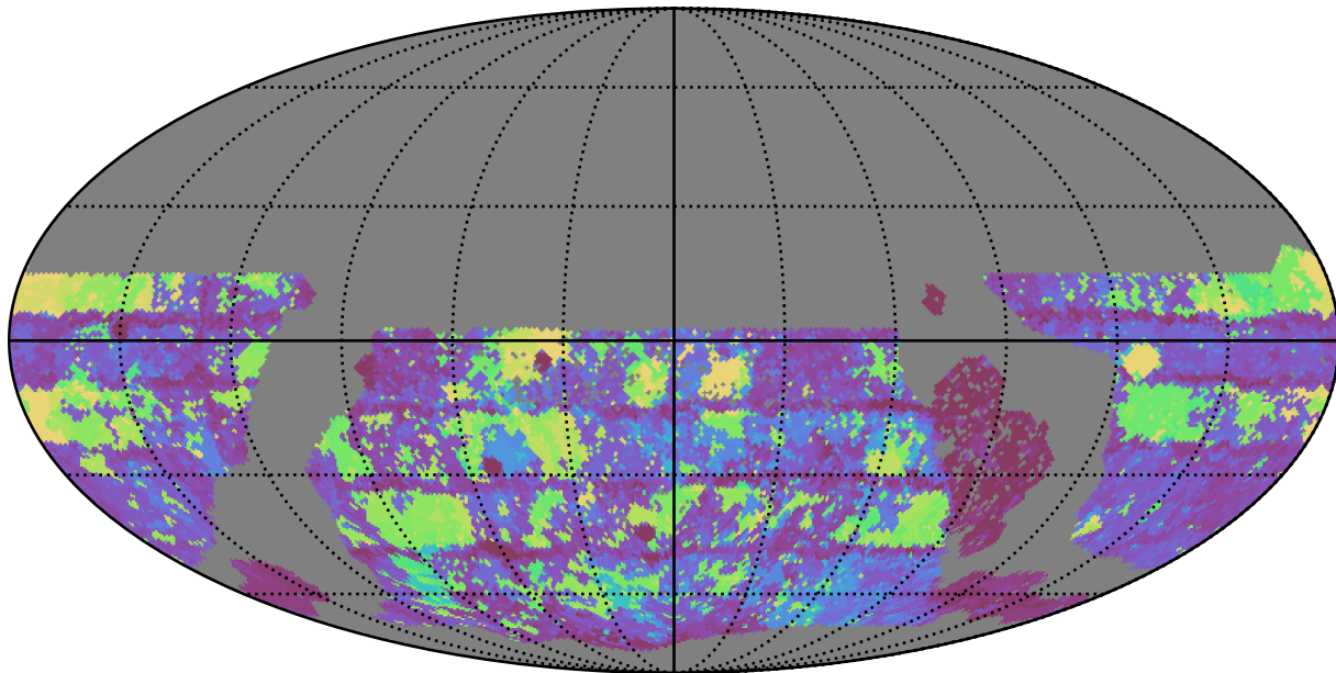
too_elab_r32_d2_giz_v3.4_10yrs WFD g band: Max Inter-Night Gap
