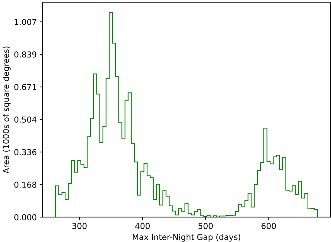
too_elab_r32_d2_giz_v3.4_10yrs WFD g band: Max Inter-Night Gap
