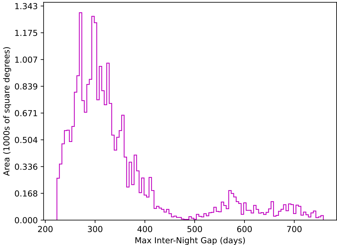
too_elab_r32_d2_giz_v3.4_10yrs All sky z band: Max Inter-Night Gap
