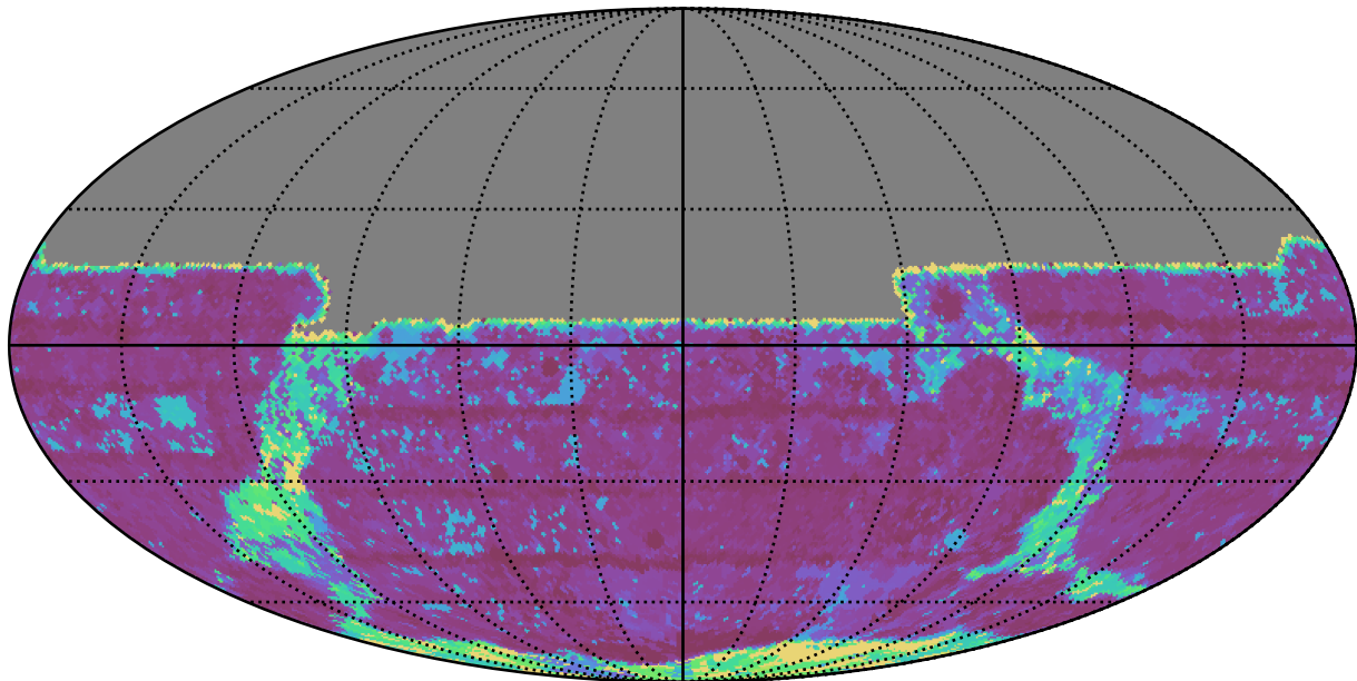
too_elab_r32_d2_giz_v3.4_10yrs All sky y band: Max Inter-Night Gap
