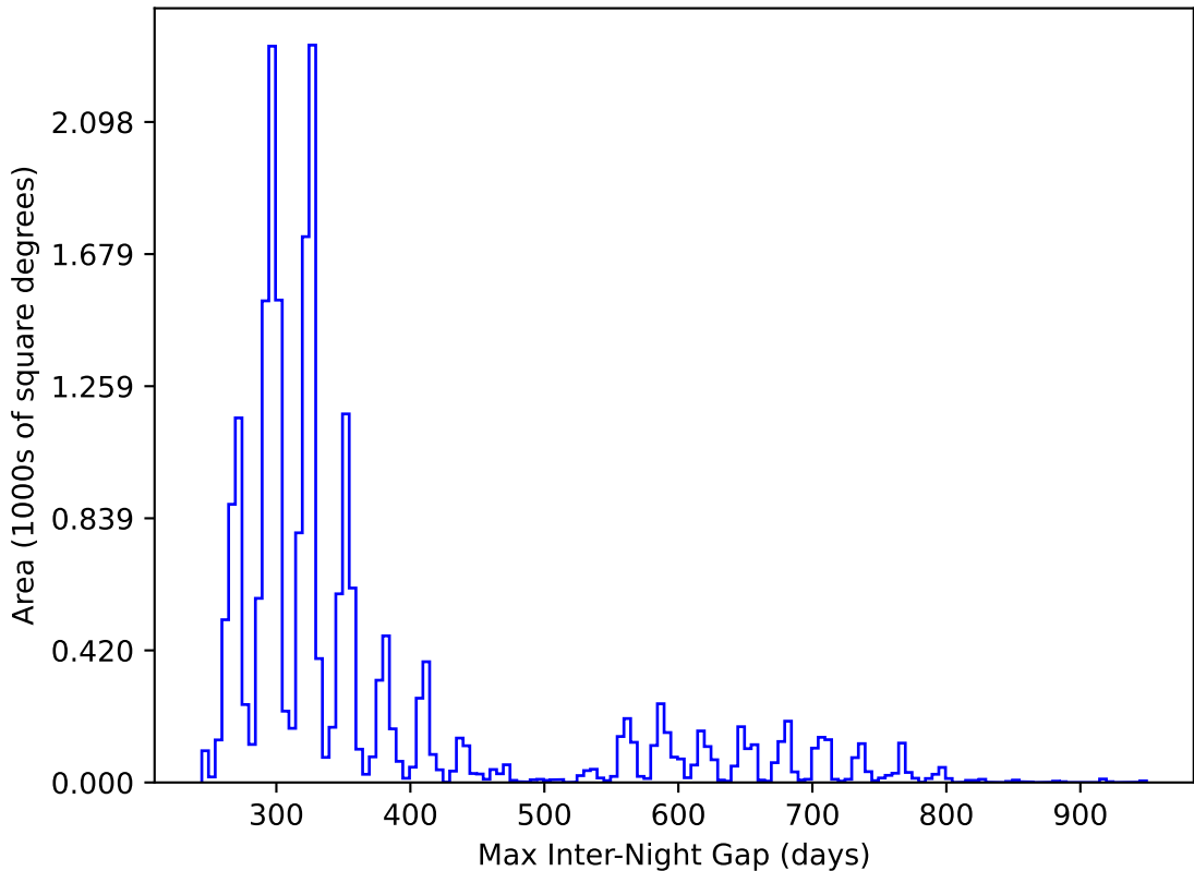
too_elab_r32_d2_giz_v3.4_10yrs All sky y band: Max Inter-Night Gap
