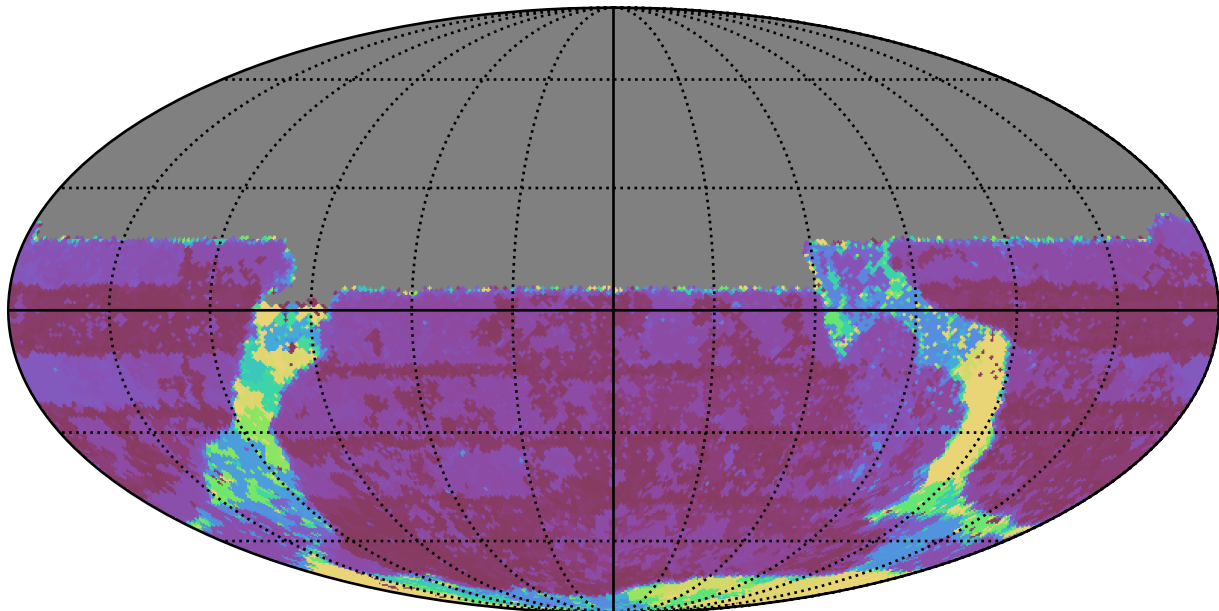
too_elab_r32_d2_giz_v3.4_10yrs All sky u band: Max Inter-Night Gap
