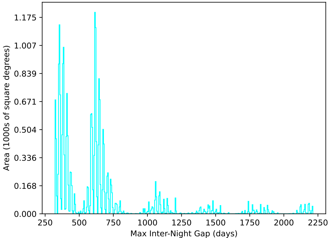
too_elab_r32_d2_giz_v3.4_10yrs All sky u band: Max Inter-Night Gap
