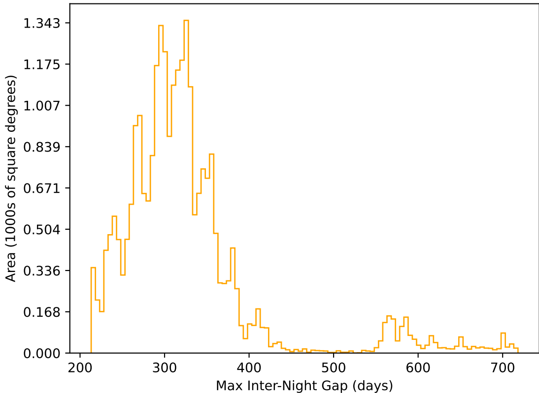
too_elab_r32_d2_giz_v3.4_10yrs All sky r band: Max Inter-Night Gap
