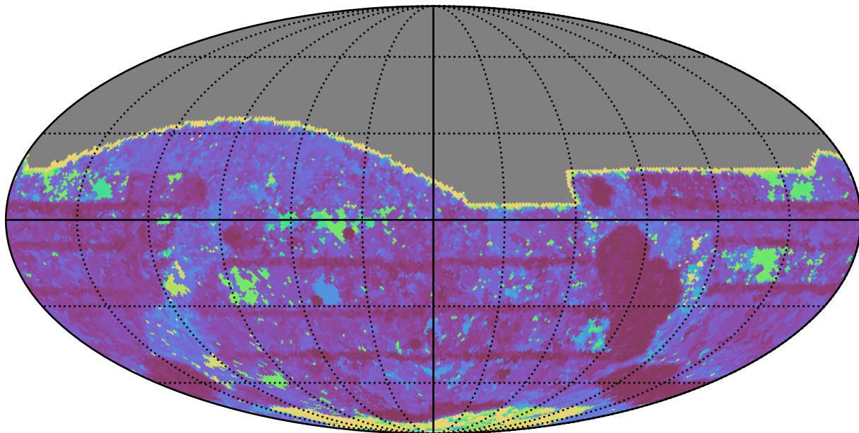
too_elab_r32_d2_giz_v3.4_10yrs All sky i band: Max Inter-Night Gap
