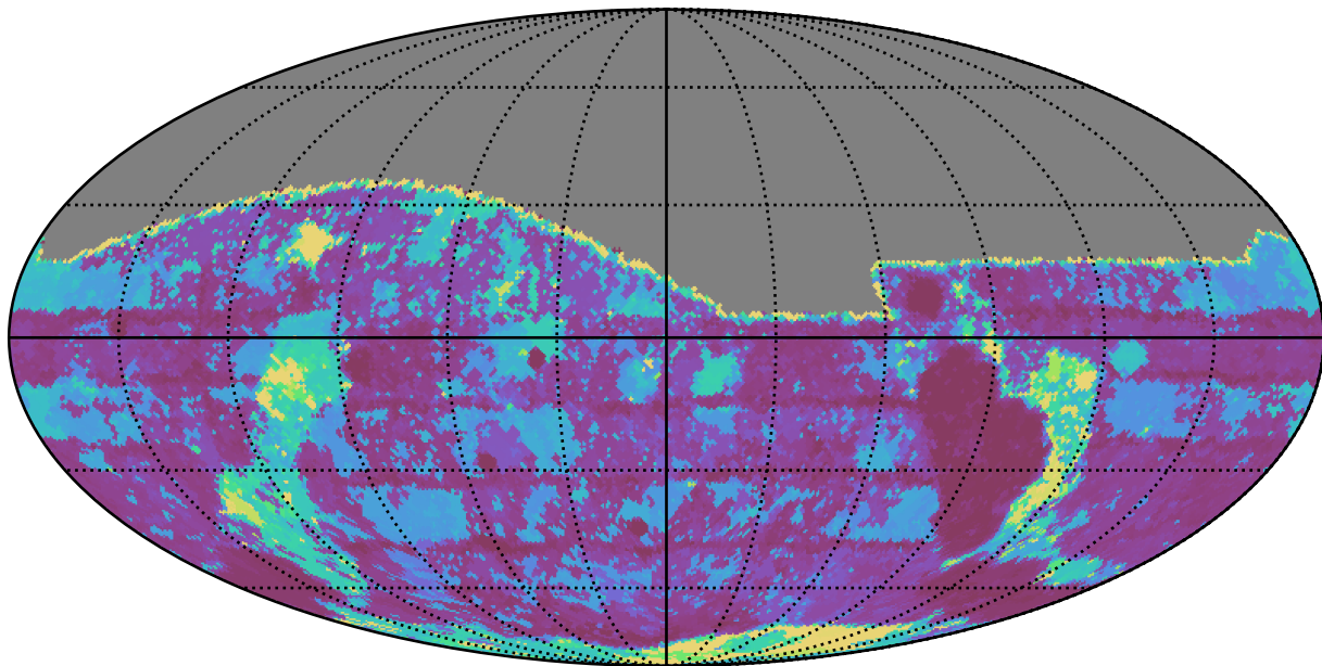
too_elab_r32_d2_giz_v3.4_10yrs All sky g band: Max Inter-Night Gap
