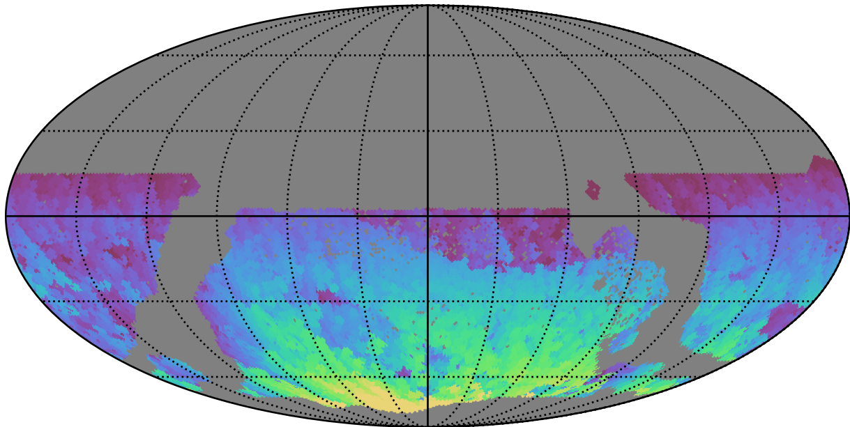
too_elab_r32_d2_giz_v3.4_10yrs WFD z band: Max HA
