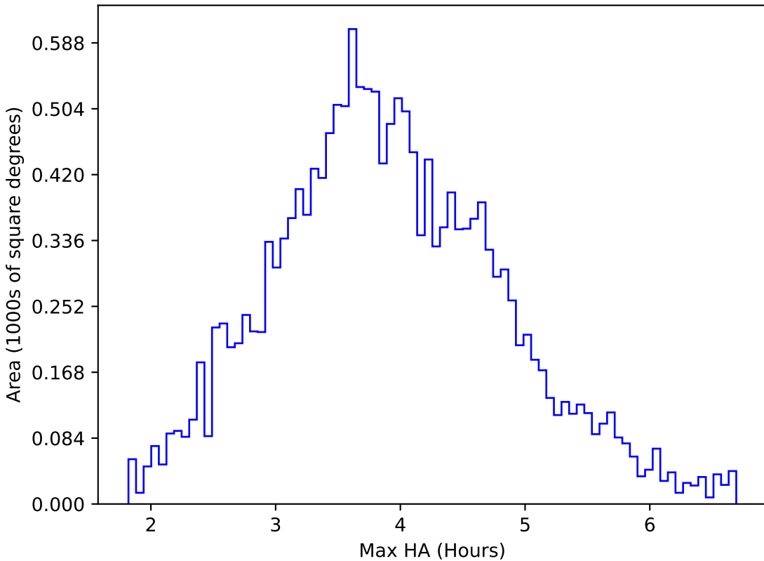
too_elab_r32_d2_giz_v3.4_10yrs WFD u band: Max HA
