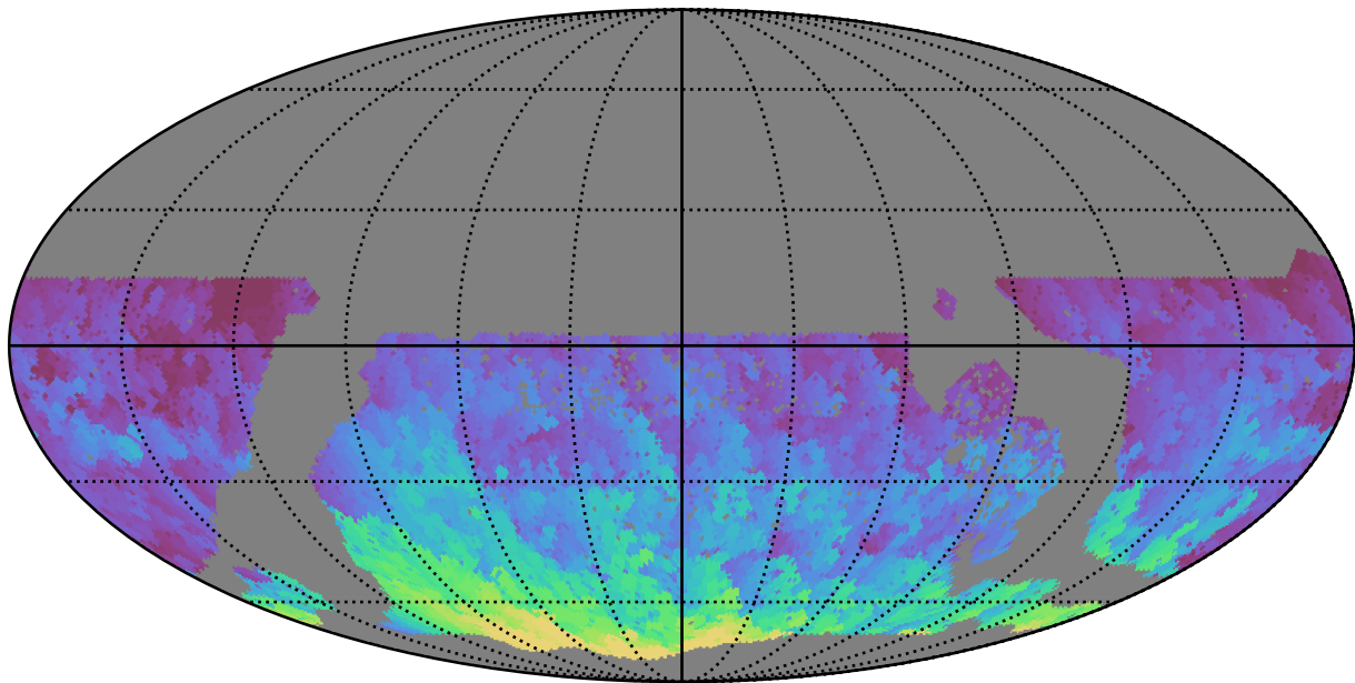
too_elab_r32_d2_giz_v3.4_10yrs WFD r band: Max HA
