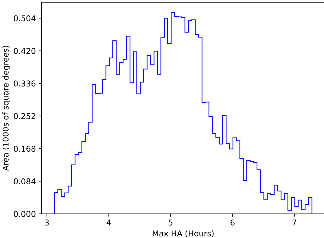
too_elab_r32_d2_giz_v3.4_10yrs WFD i band: Max HA
