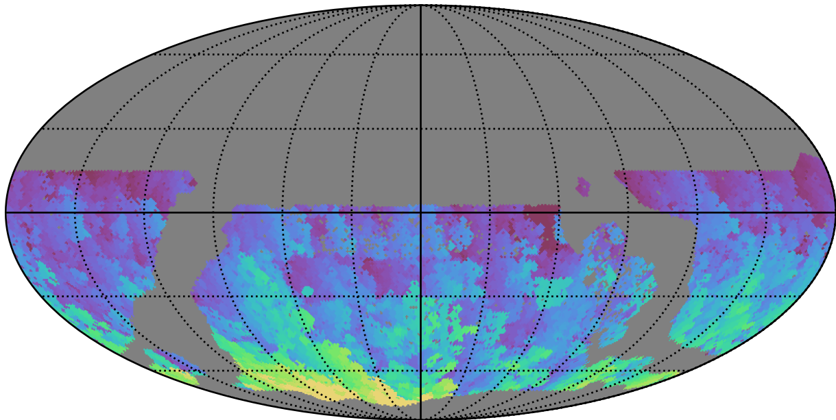
too_elab_r32_d2_giz_v3.4_10yrs WFD g band: Max HA
