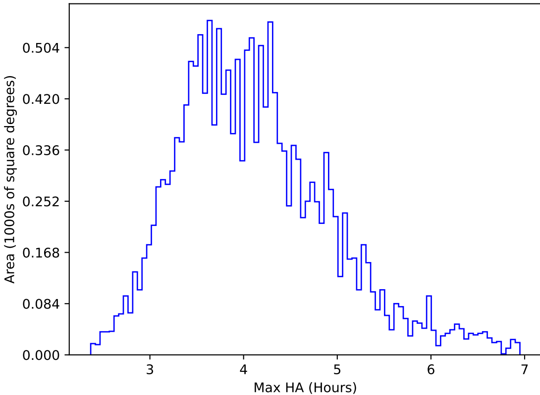
too_elab_r32_d2_giz_v3.4_10yrs WFD g band: Max HA
