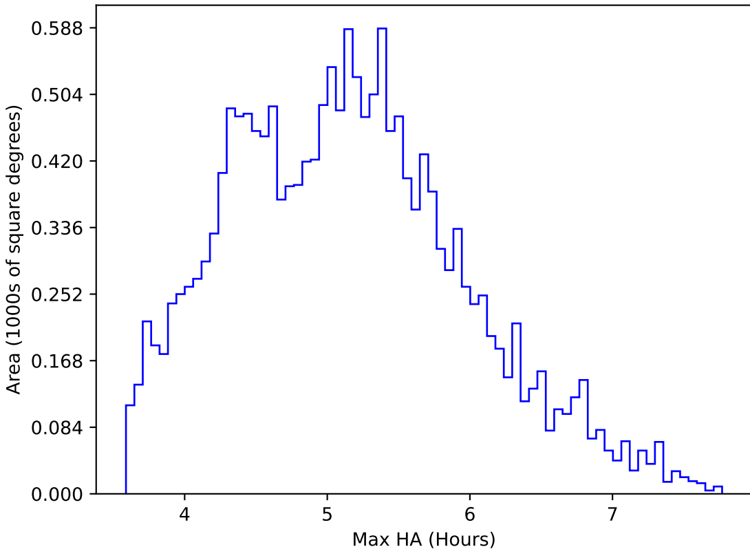
too_elab_r32_d2_giz_v3.4_10yrs WFD all bands: Max HA
