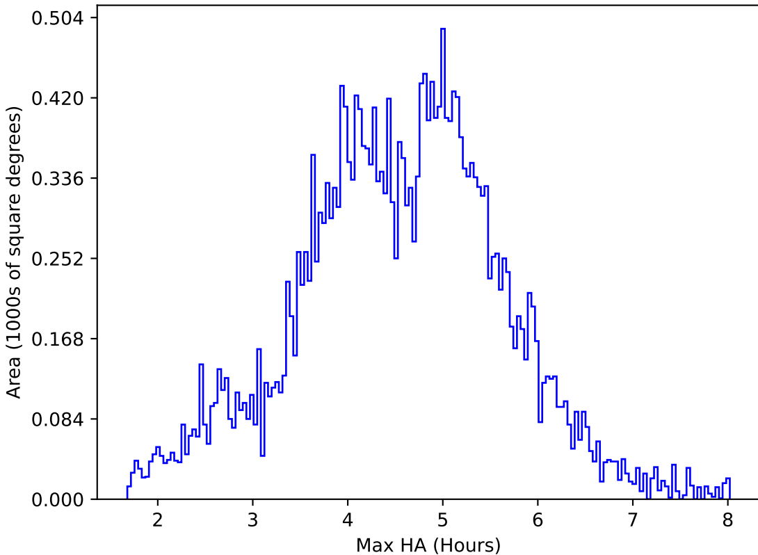
too_elab_r32_d2_giz_v3.4_10yrs All sky z band: Max HA
