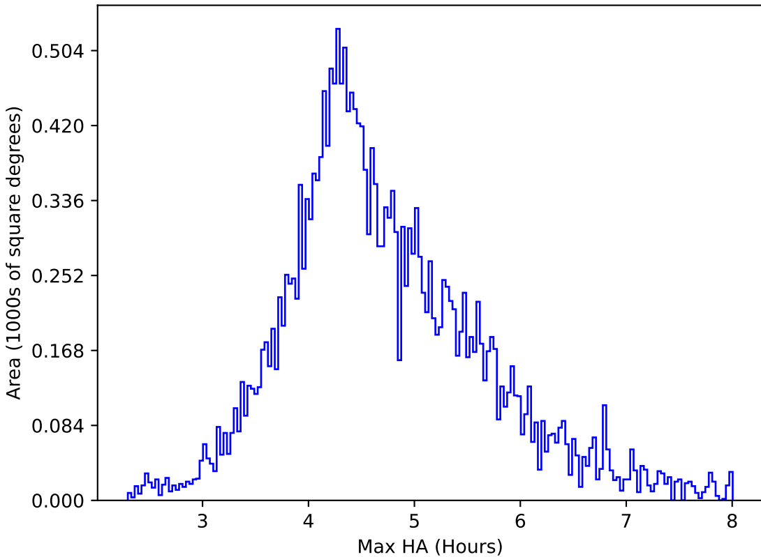
too_elab_r32_d2_giz_v3.4_10yrs All sky y band: Max HA
