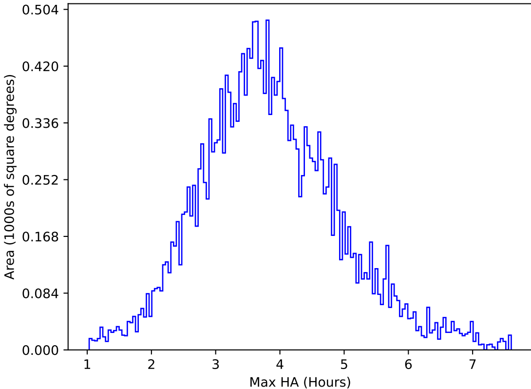
too_elab_r32_d2_giz_v3.4_10yrs All sky u band: Max HA
