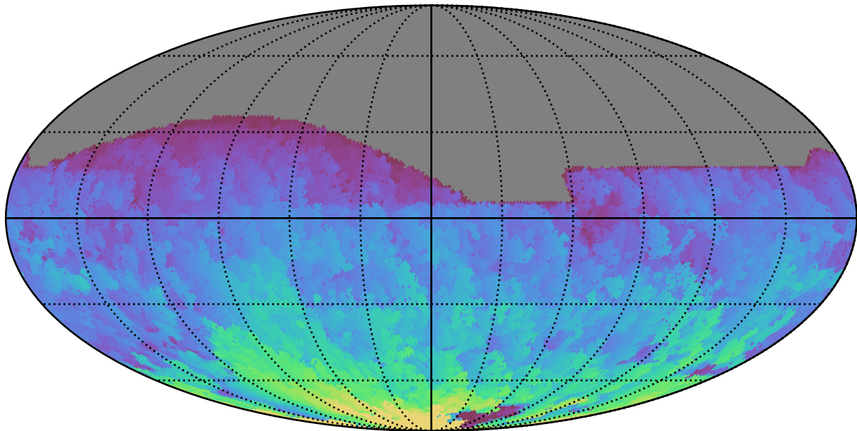
too_elab_r32_d2_giz_v3.4_10yrs All sky r band: Max HA
