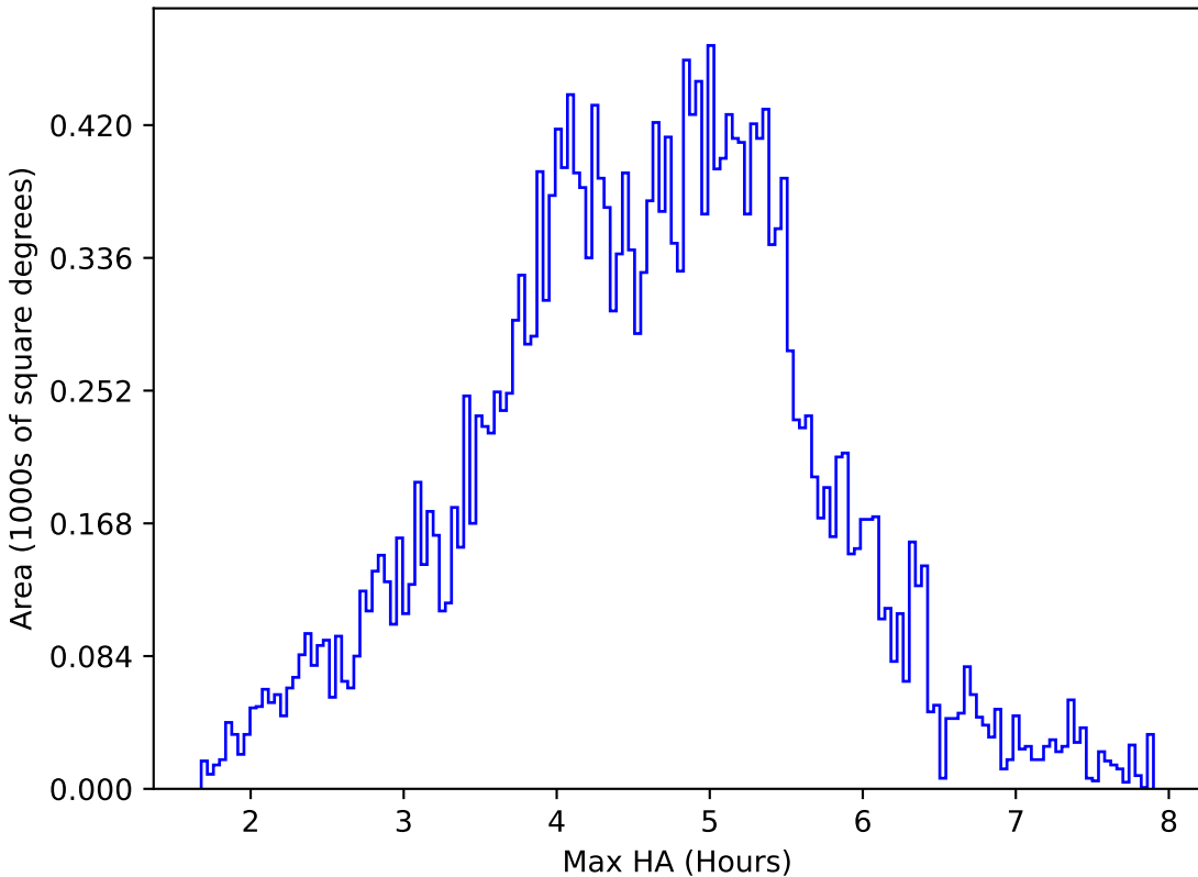
too_elab_r32_d2_giz_v3.4_10yrs All sky i band: Max HA
