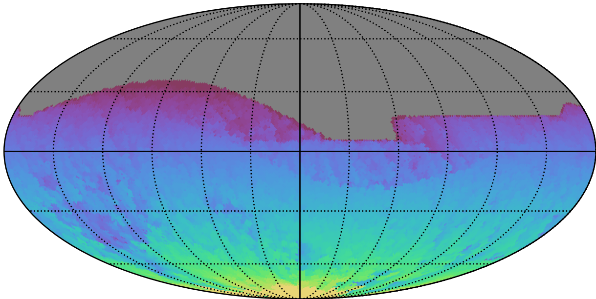
too_elab_r32_d2_giz_v3.4_10yrs All sky all bands: Max HA
