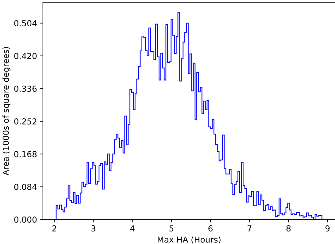
too_elab_r32_d2_giz_v3.4_10yrs All sky all bands: Max HA
