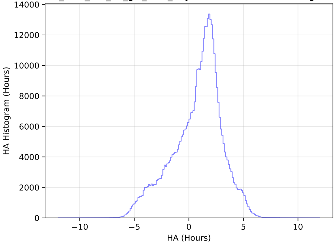
too_elab_r32_d2_giz_v3.4_10yrs WFD z band: HA Histogram
