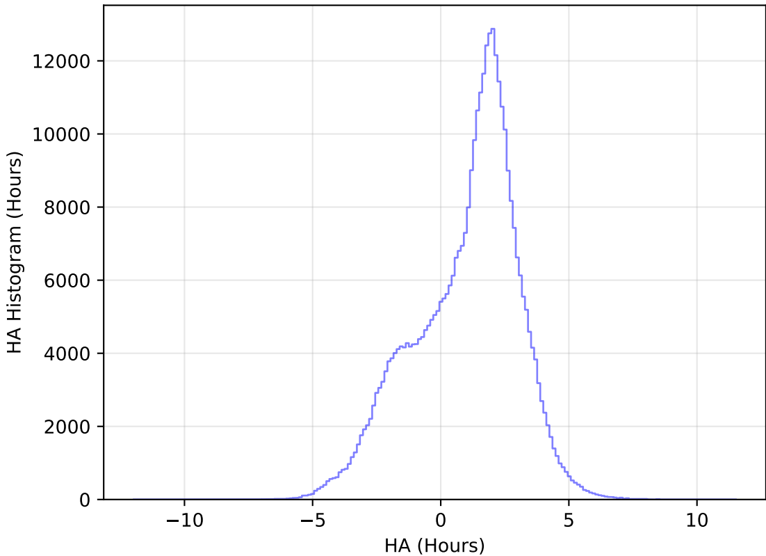
too_elab_r32_d2_giz_v3.4_10yrs WFD y band: HA Histogram
