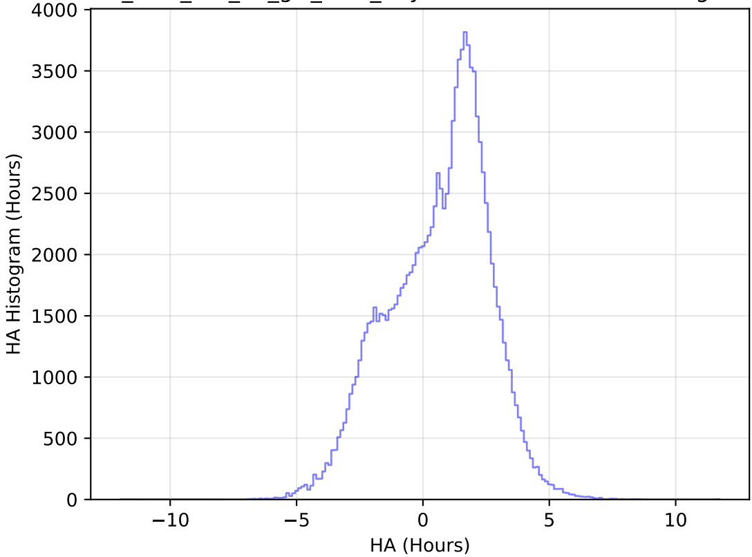
too_elab_r32_d2_giz_v3.4_10yrs WFD u band: HA Histogram
