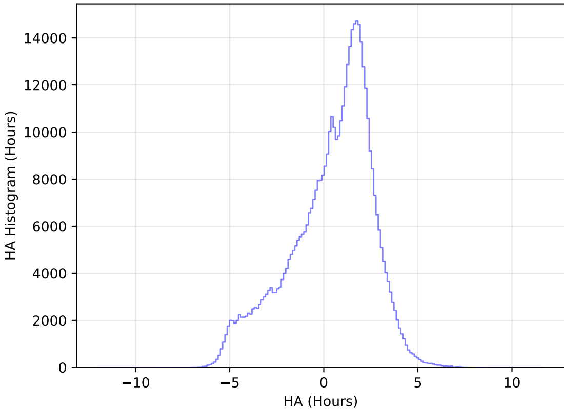
too_elab_r32_d2_giz_v3.4_10yrs WFD r band: HA Histogram
