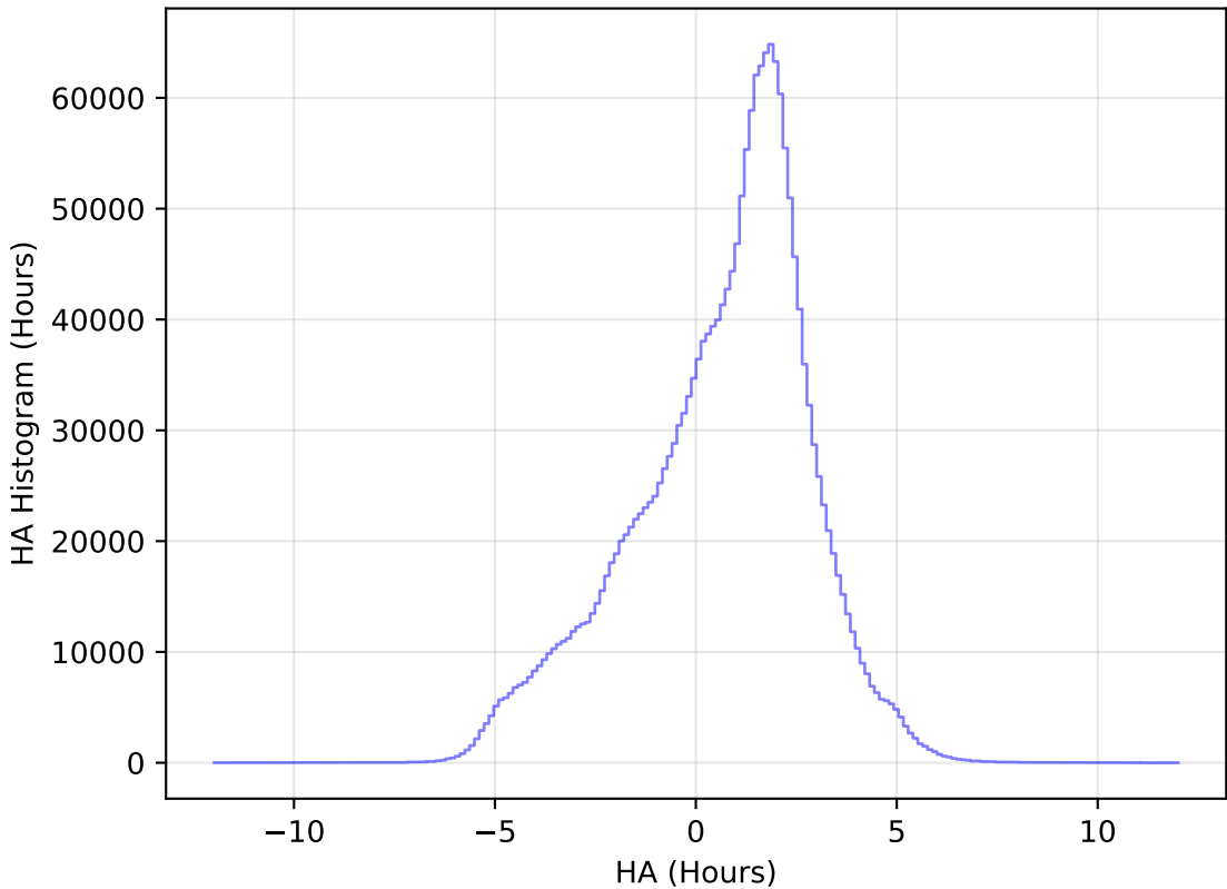
too_elab_r32_d2_giz_v3.4_10yrs WFD all bands: HA Histogram
