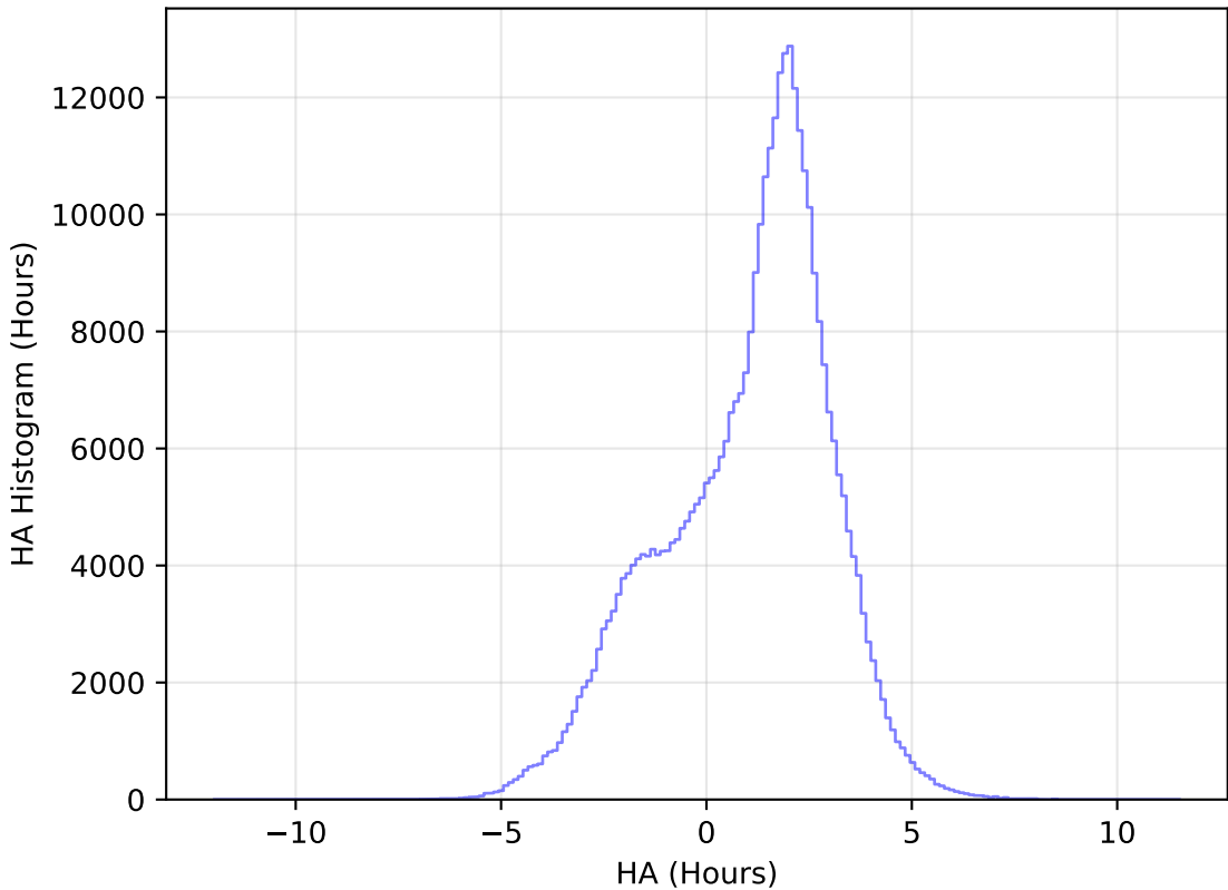
too_elab_r32_d2_giz_v3.4_10yrs All sky y band: HA Histogram
