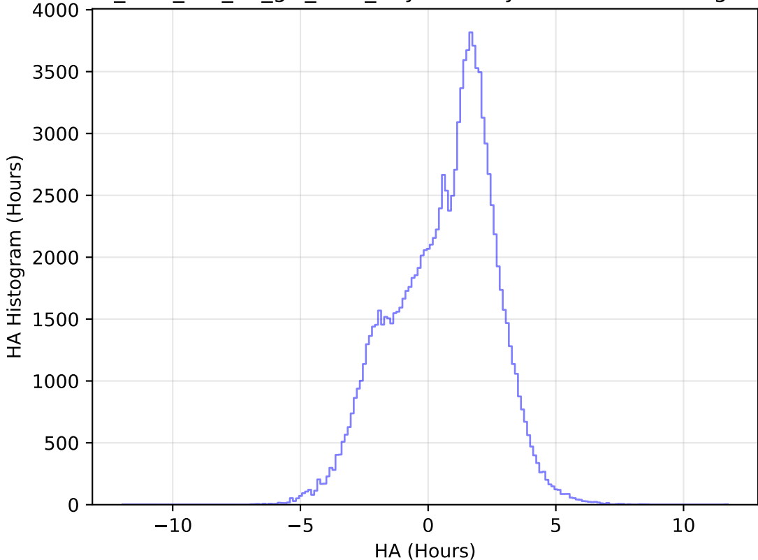
too_elab_r32_d2_giz_v3.4_10yrs All sky u band: HA Histogram
