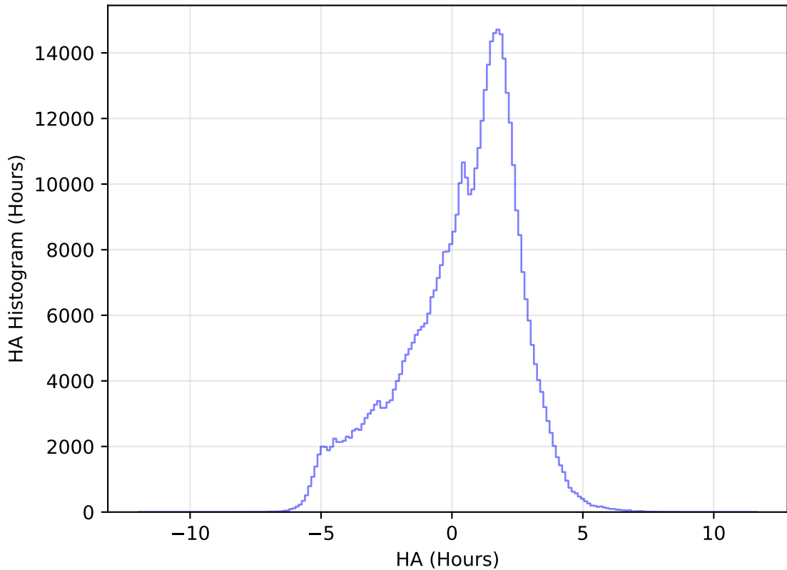
too_elab_r32_d2_giz_v3.4_10yrs All sky r band: HA Histogram
