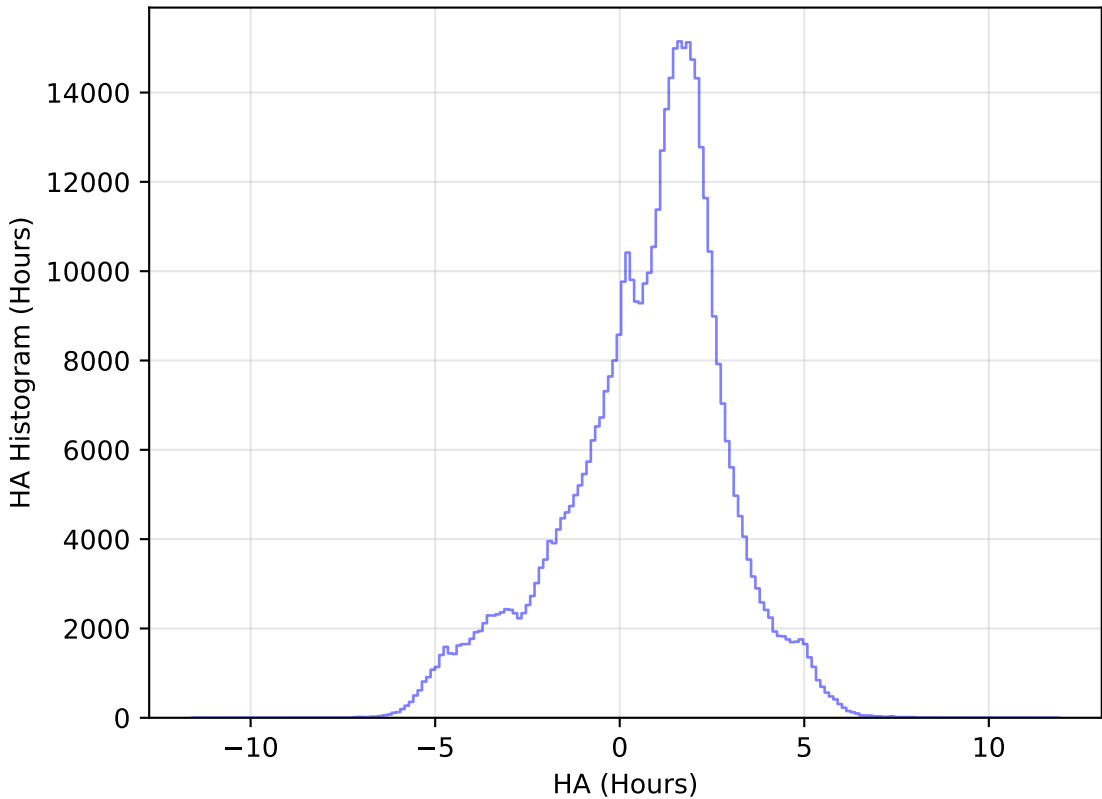
too_elab_r32_d2_giz_v3.4_10yrs All sky i band: HA Histogram
