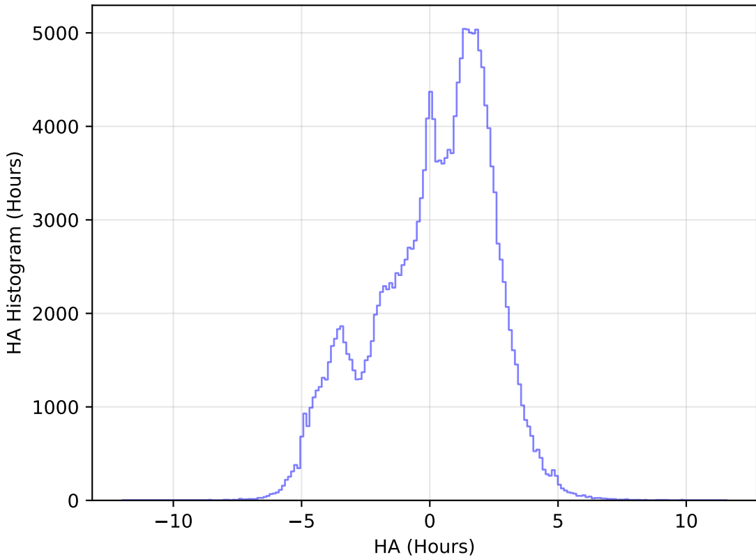
too_elab_r32_d2_giz_v3.4_10yrs All sky g band: HA Histogram
