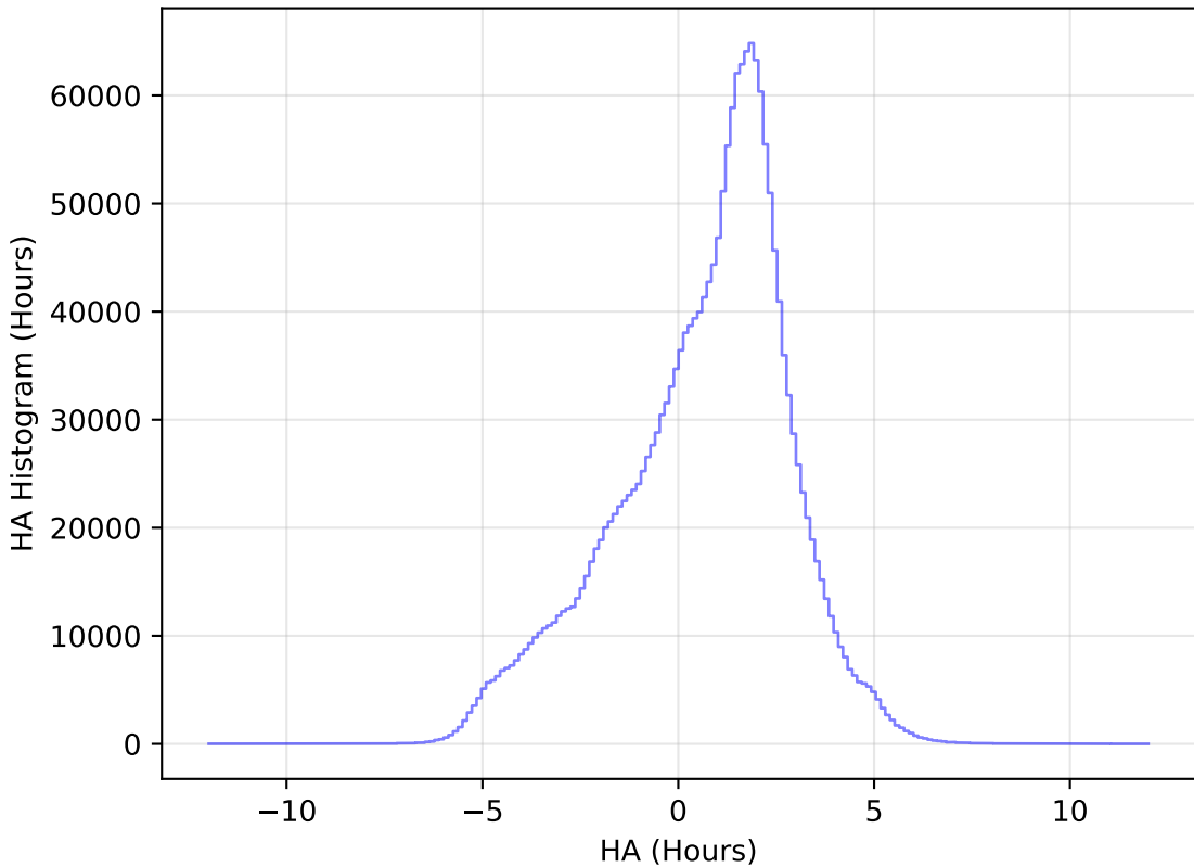
too_elab_r32_d2_giz_v3.4_10yrs All sky all bands: HA Histogram
