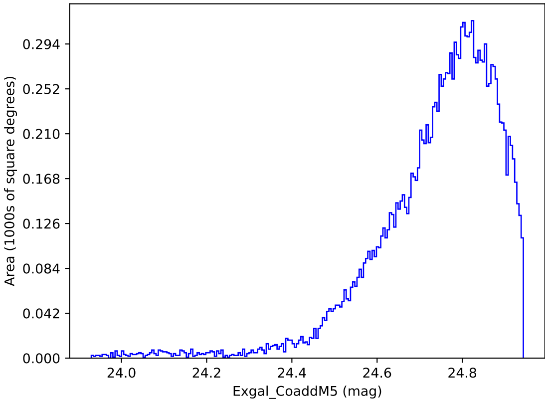
too_elab_r32_d2_giz_v3.4_10yrs WFD y band: Exgal_CoaddM5
