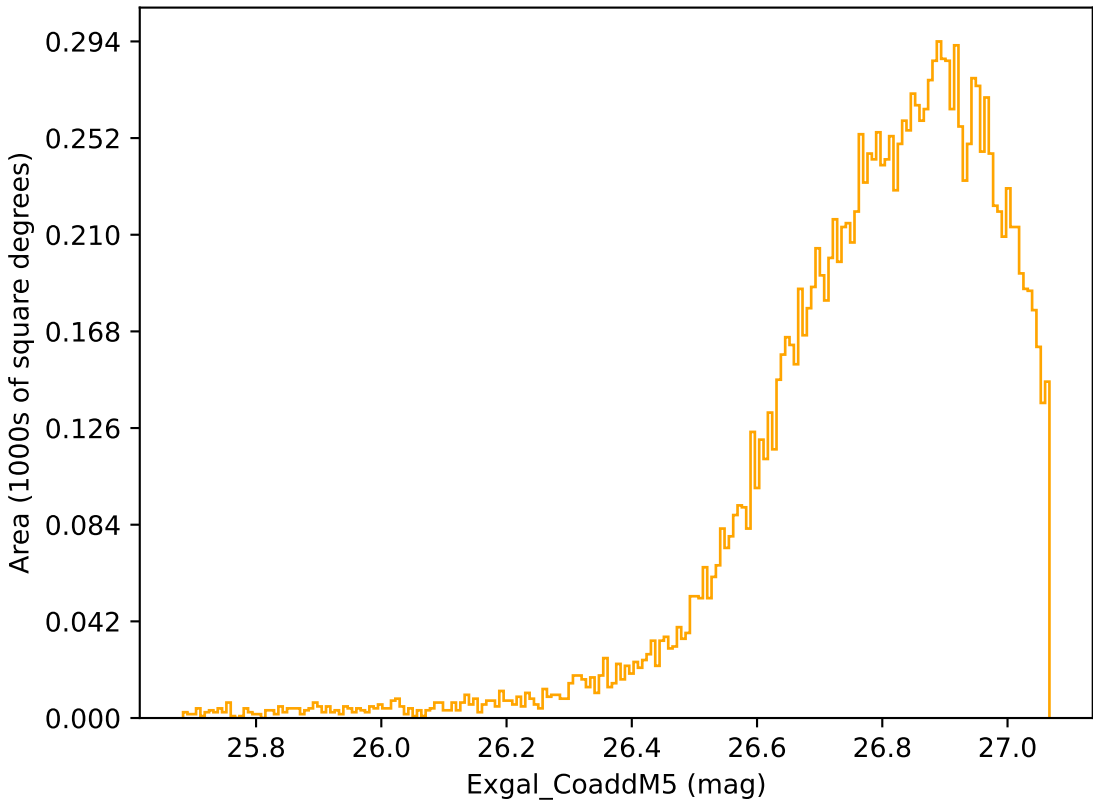
too_elab_r32_d2_giz_v3.4_10yrs WFD r band: Exgal_CoaddM5
