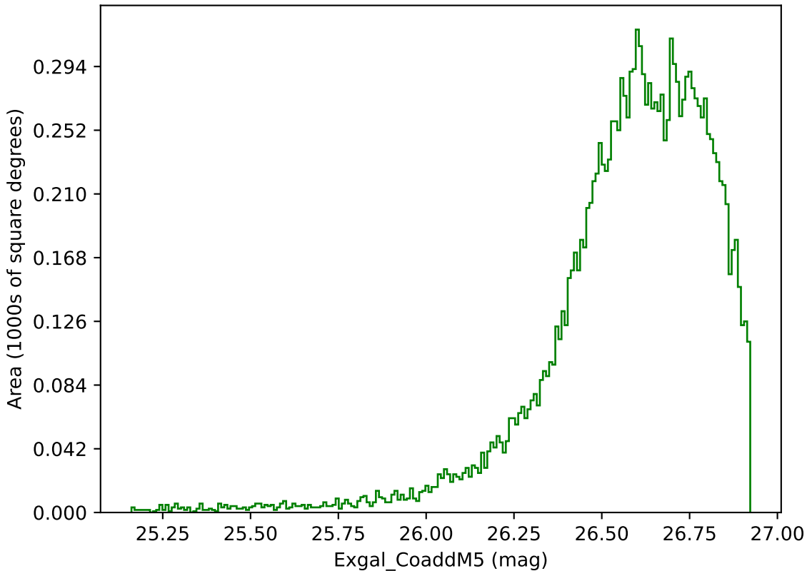
too_elab_r32_d2_giz_v3.4_10yrs WFD g band: Exgal_CoaddM5
